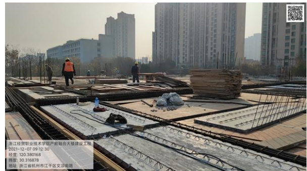
(PC 叠合板安装)
